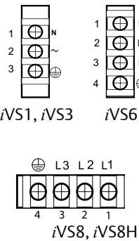
Figure 1. AC Input
