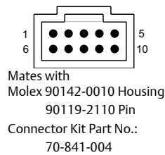
Figure 2. Connector J1
