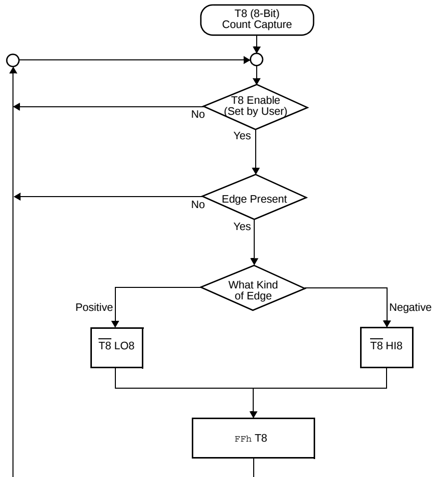
Figure 18. DEMODULATION Mode Count Capture Flowchart
