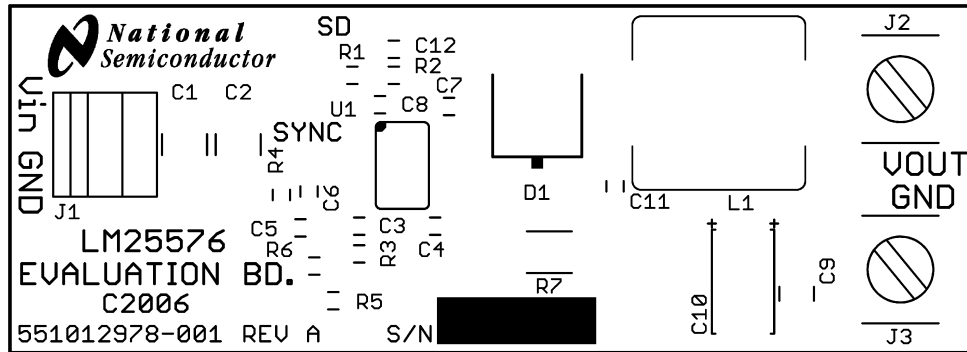
Figure 23. Silkscreen
