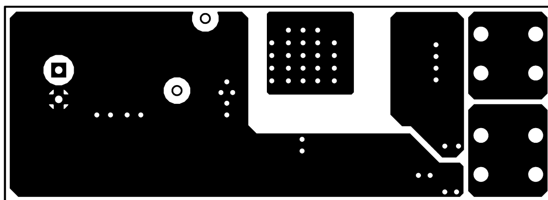
Figure 22. Solder Side
