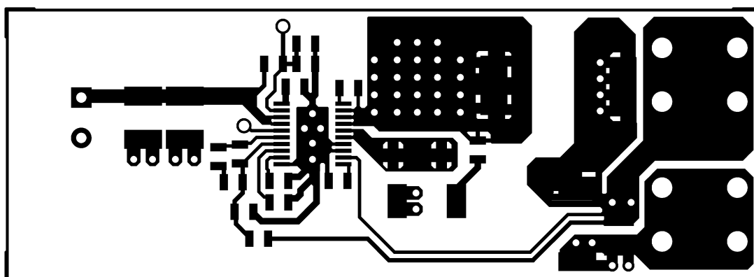
Figure 21. Component Side
