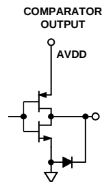
Figure 22. Comparator Outputs
