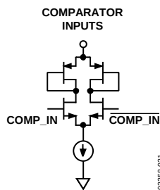
Figure 21. Comparator Inputs
