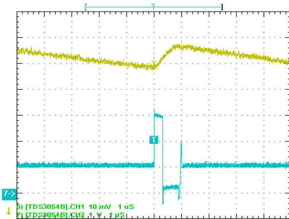
Ripple in DCM: Fripple = 145kHz, Vin = 2.85V, Vout = 0.85V, Iout = 10mA Ripple = 10mV (worst case), 1 \mu s/DIV
