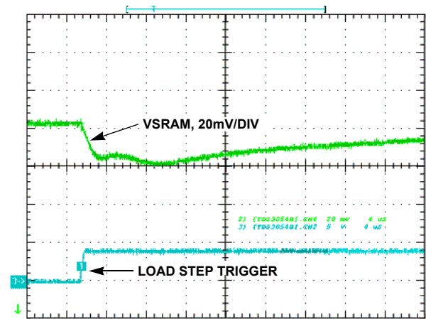
LDO transient response with 3.3 \mu F output capacitance. LVCC = 4.1V. 10mA DC load+ 55mA step load.
