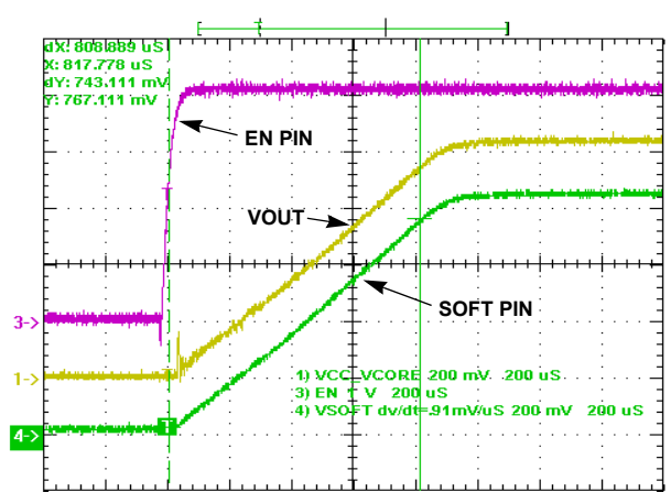
Soft-start into CCM, VIN = 4.2V, CH3 = EN pin. Vout = 0.85 Soft-Start capacitor = 10nF. 200 \mu s/DIV
