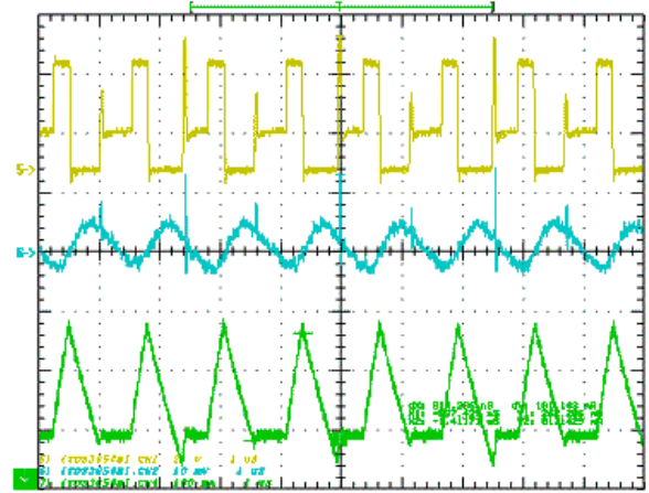
Top: phase node output voltage ripple, 10mV/DIV Bottom: Inductor current, 100mA/DIV, 1 \mu s/DIV
