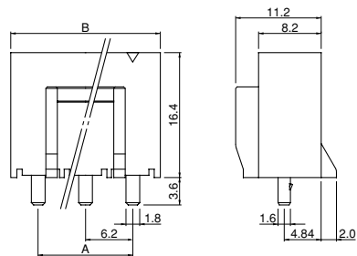
(2, 3 circuits)
