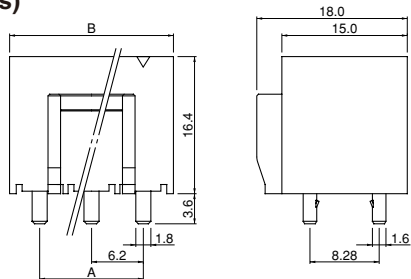
(Single-row 4 circuits)
