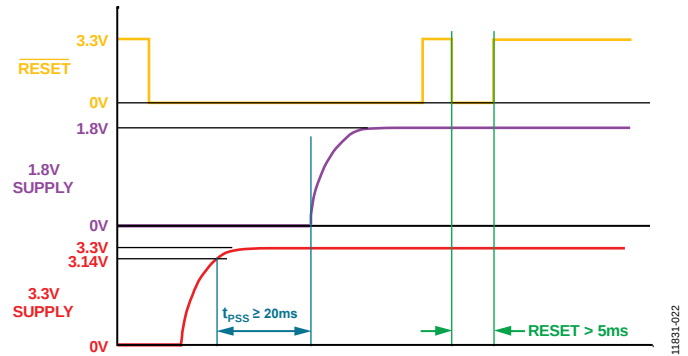
Figure 20. ADV7625 Supply Power-Up Sequence
