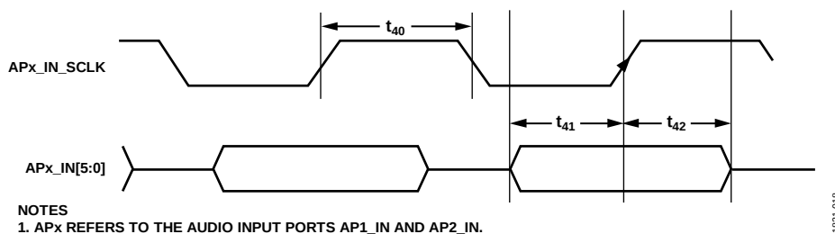
Figure 16. DSD Input Timing
