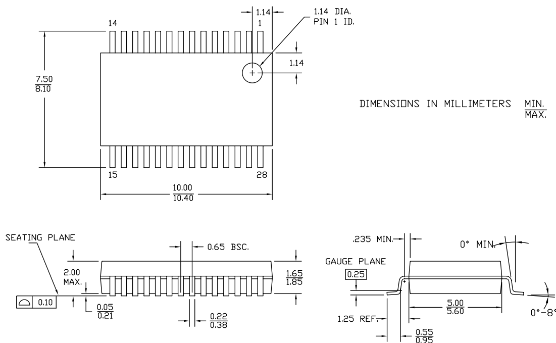
Figure 17. 28-pin SSOP (210 Mils) O28.21 Package Outline, 51-85079
