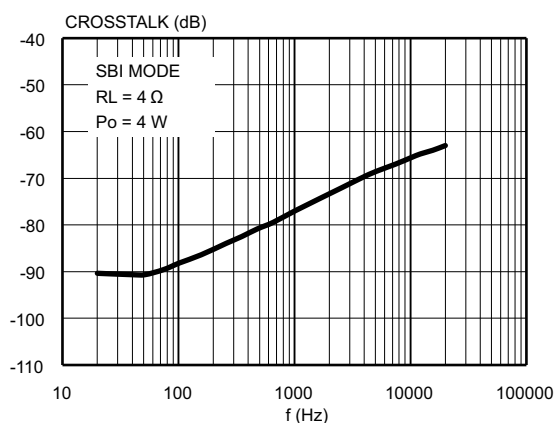
Figure 21. Crosstalk vs. frequency (SBI mode)
