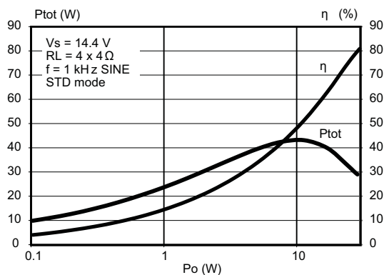
Figure 23. Total power dissipation & efficiency vs. P_o (4 Ω, STD, Sine)
