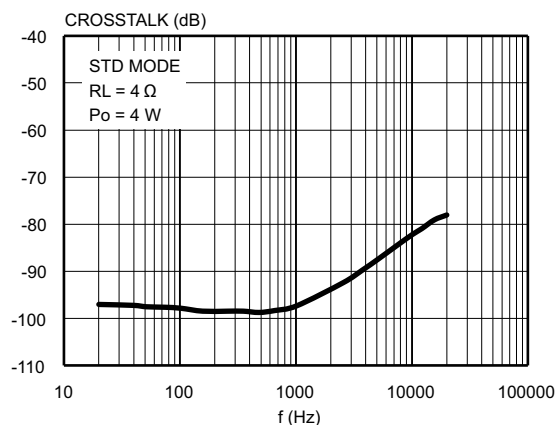
Figure 20. Crosstalk vs. frequency (STD mode)
