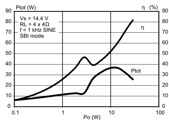
Figure 24. Total power dissipation & efficiency vs. P_o (4 Ω, SBI, Sine)
