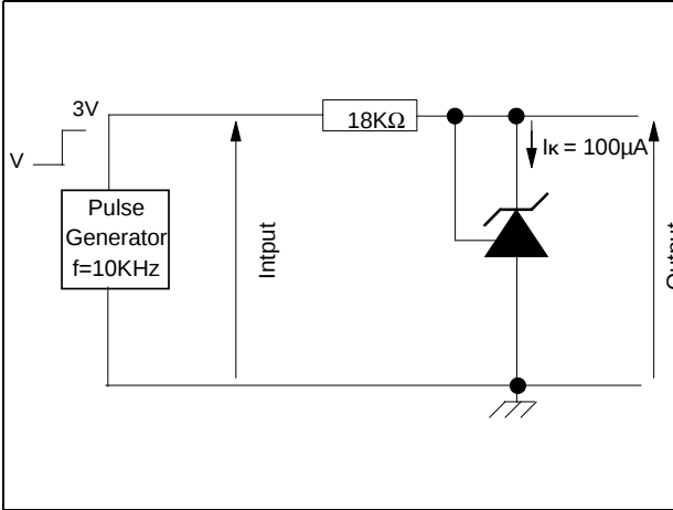
Figure 13. Test circuit for pulse response at I_K=100\mu\text{A}
