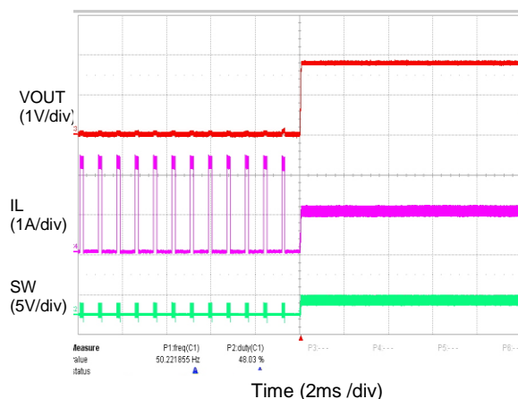
Load Transient (I OUT =0.5A to 1A)
