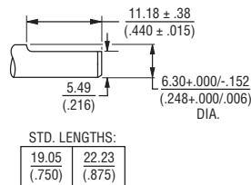
SHAFT TYPE "C" (USES BUSHING A)
