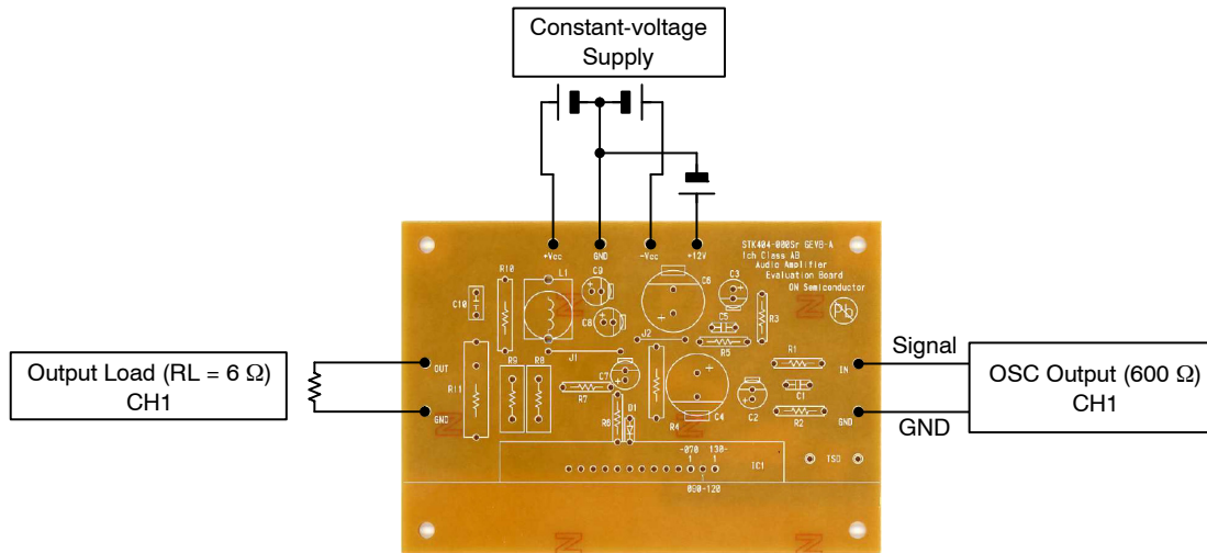
Figure 5. Characteristics Confirmation
