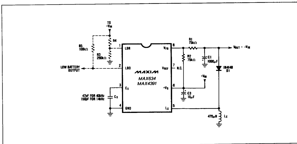
Figure 5. Regulated Voltage Inverter
