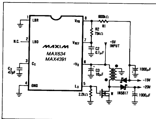
Figure 8. High Power +5V to -15V DC-DC Converter
