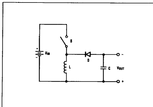
Figure 1. Simplified Voltage Inverter
