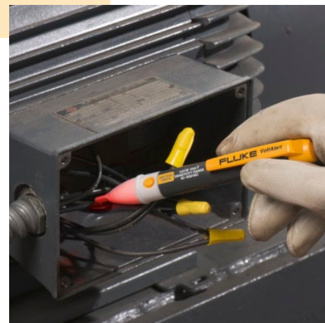
Junction box
