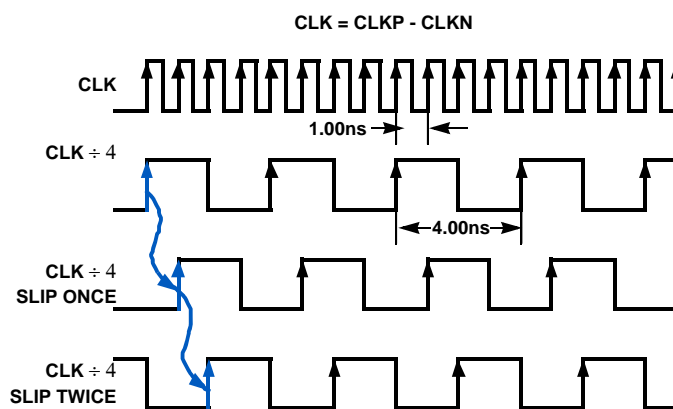
FIGURE 40. PHASE SLIP: CLK ÷ 4 MODE, f CLK = 1000MHz
