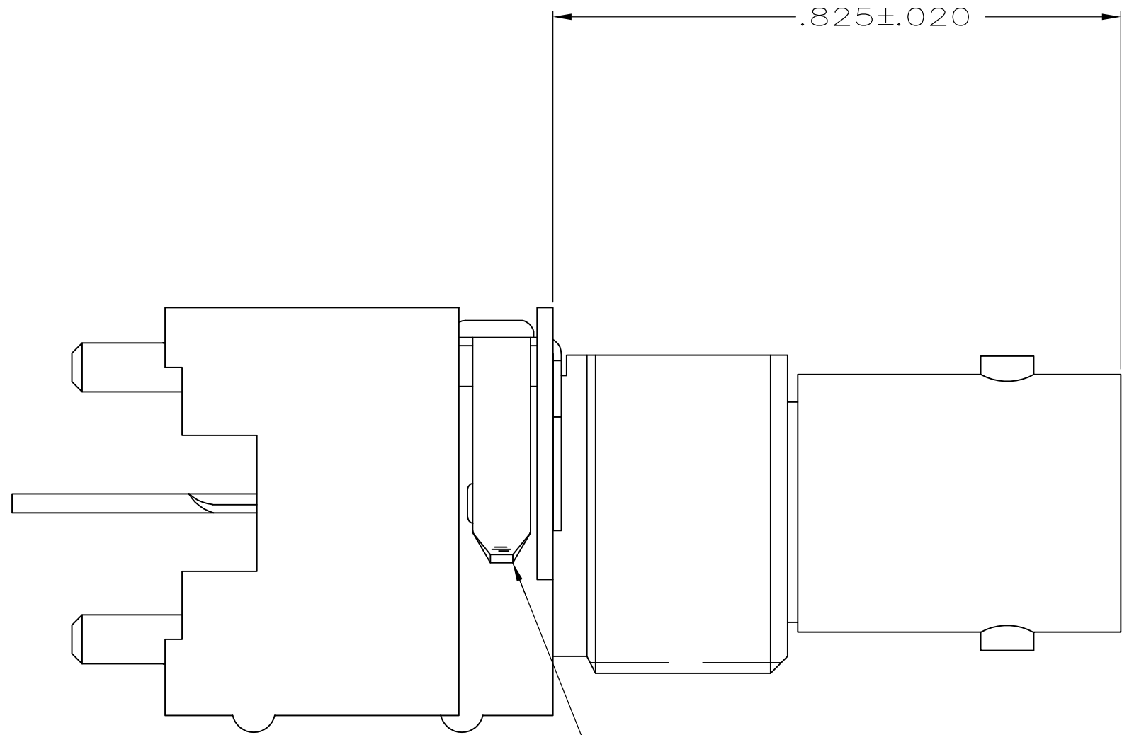
VIEW X
