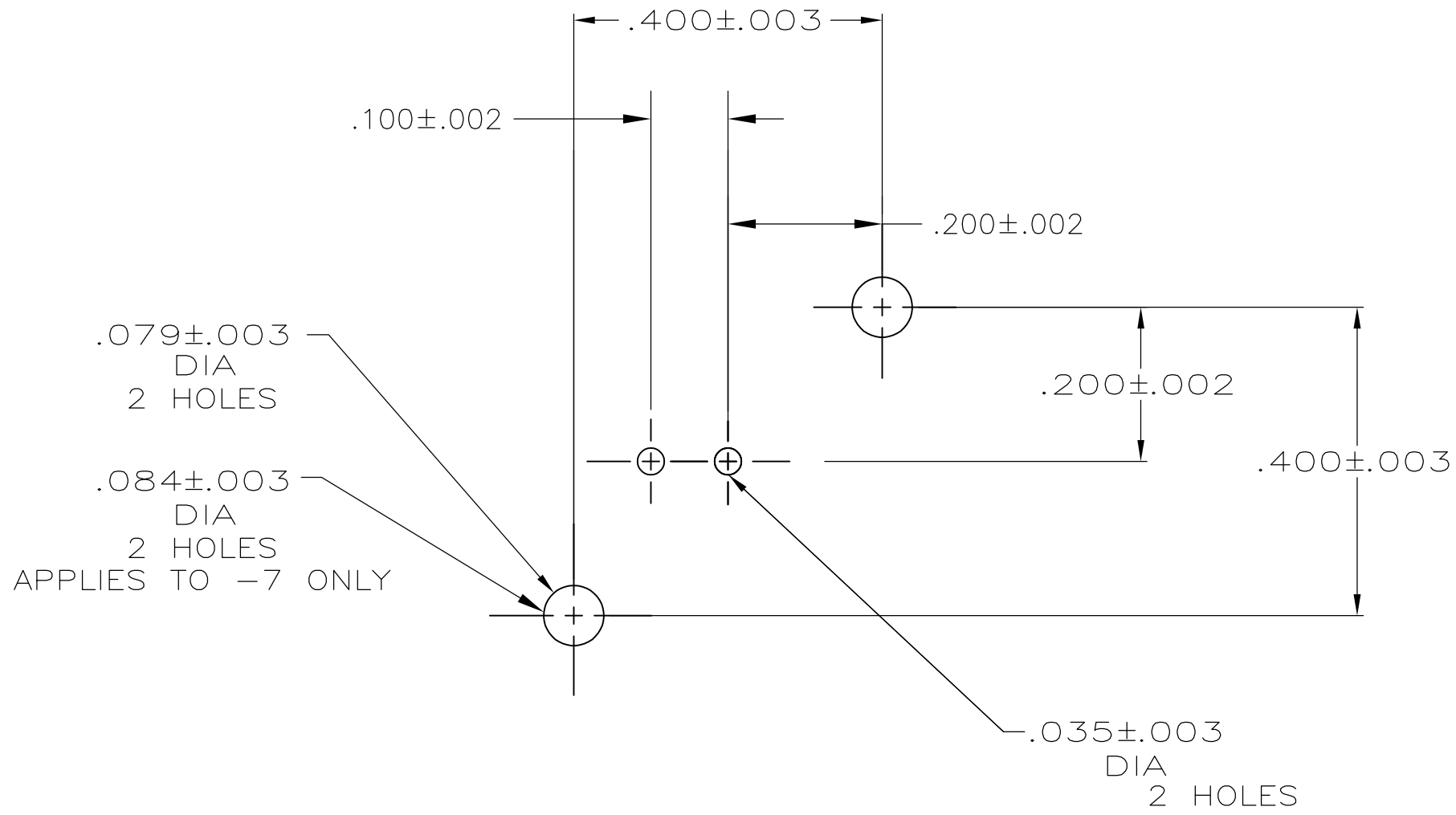
PCB CONFIGURATION
