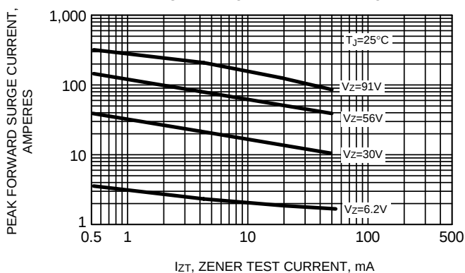
FIG. 2 - TYPICAL ZENER IMPEDANCE
