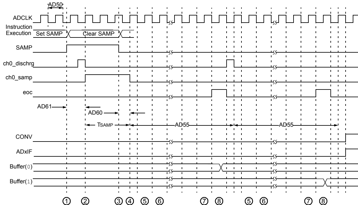
FIGURE 30-18: ANALOG-TO-DIGITAL CONVERSION (10-BIT MODE) TIMING CHARACTERISTICS (ASAM = 0, SSRC<2:0> = 000)
