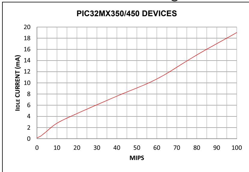
FIGURE 31-9: TYPICAL I_{IDLE} CURRENT @ V_{DD} = 3.3V
