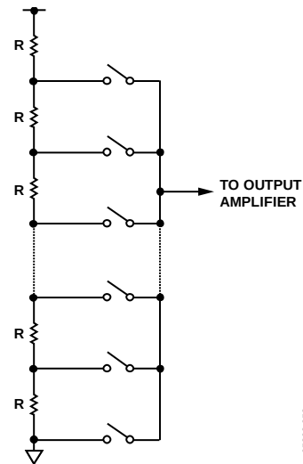
Figure 56. Resistor String
