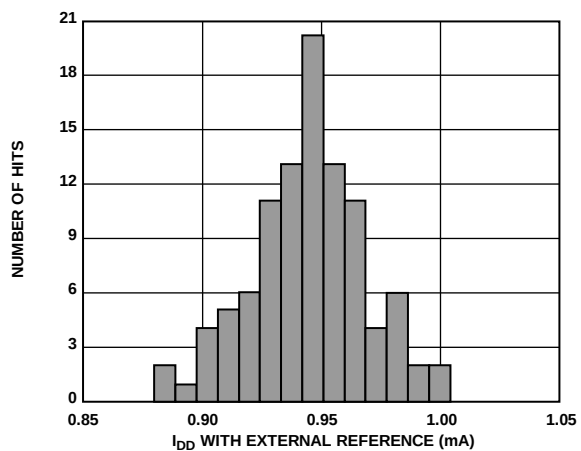
Figure 29. I_{DD} Histogram with External Reference
