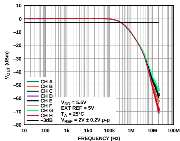
Figure 52. Multiplying Bandwidth
