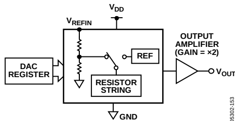
Figure 55. DAC Architecture
