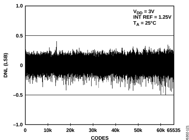
Figure 22. DNL AD5668-1
