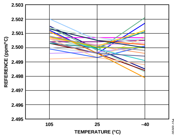
Figure 54. 2.5 V Reference Temperature Coefficient vs. Temperature
