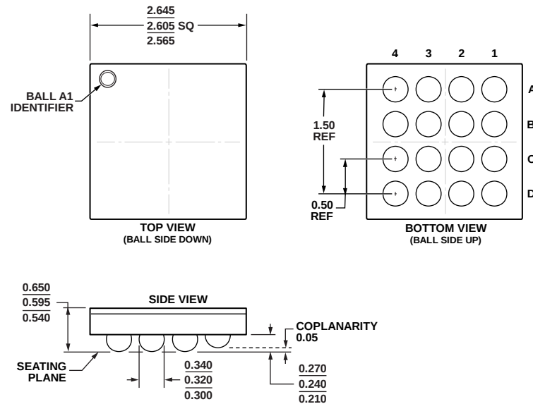
Figure 65. 16-Ball Wafer Level Chip Scale Package [WLCSP] (CB-16-16) Dimensions shown in millimeters
