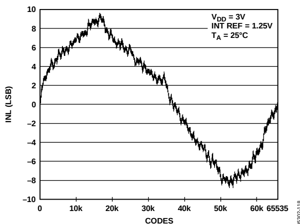
Figure 19. INL AD5668-1
