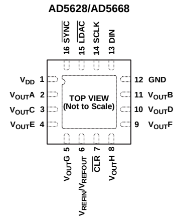
Figure 5. 16-Lead LFCSP (CP-16-17)
