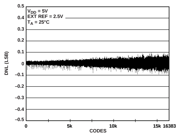
Figure 17. DNL AD5648-2
