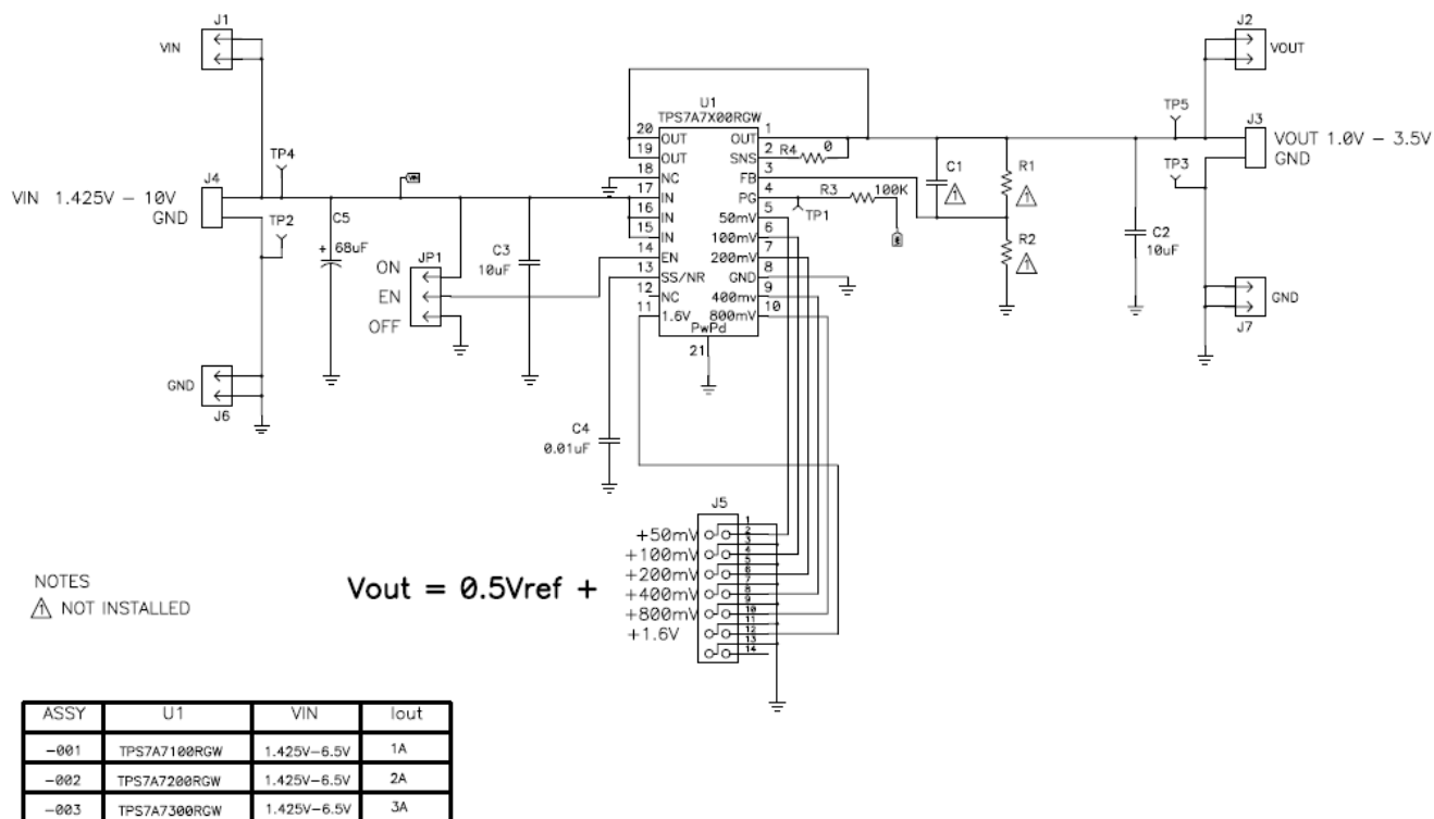
Figure 6. TPS7A7x00EVM-718 Schematic
