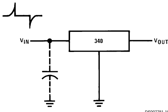
FIGURE 3. Transients
