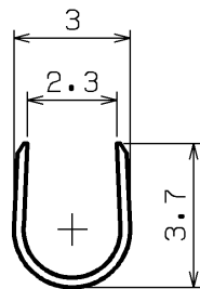
INSULATION BARREL
