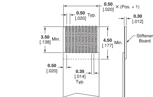
Recommended FPC Layout
