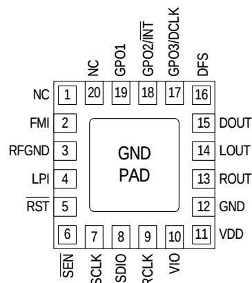
Si4704/05-GM (Top View)
