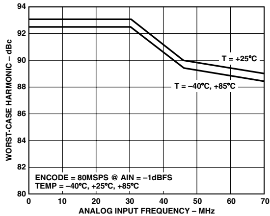
TPC 8. Harmonics vs. Analog Frequency
