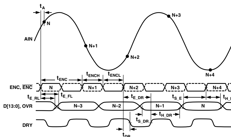
Figure 1. Timing Diagram
