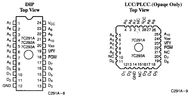
Figure 1. Programming Pinouts
