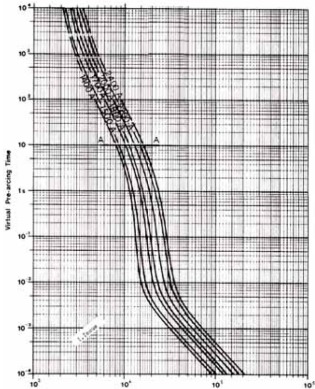
Size 4 — 1400-2400A: 1250V Time-Current Curve
