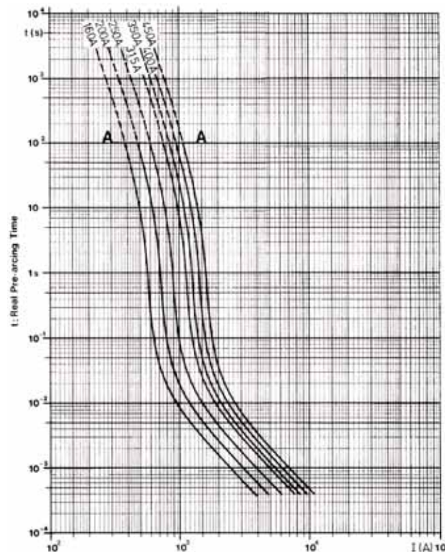
Square Body DC Fuses — 160-450A: 4000V Time-Current Curve
