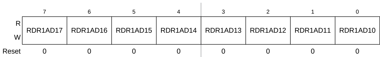
Figure 24-65. Port AD1 Reduced Drive Register 1 (RDR1AD1)
