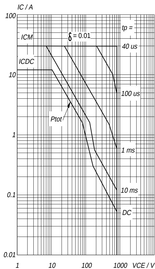
Fig.15. Forward bias safe operating area. T_{mb} = 25\text{ }^{\circ}\text{C} I_{CD} & I_{CM} = f(V_{CE}) ; I_{CM} single pulse; parameter t_p ; Second-breakdown limits independent of temperature.
