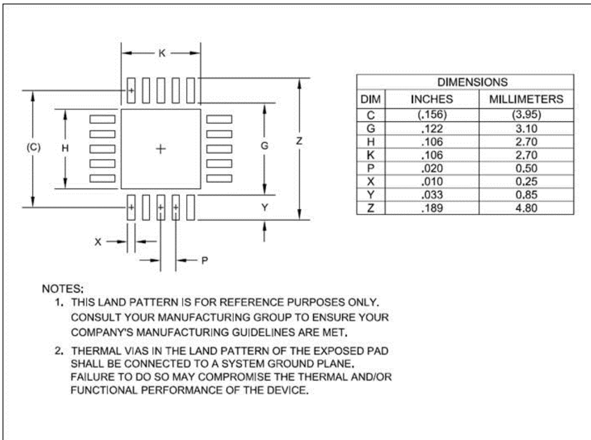
Figure 8: Recommended Board Layout Land Pattern
