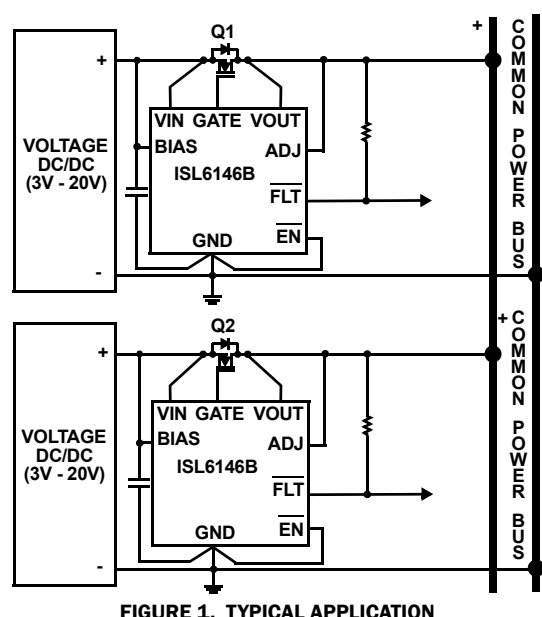
FIGURE 1. TYPICAL APPLICATION
