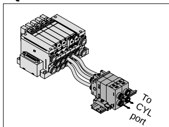
Double check block (Separated) VVQ2000-FPG-□□-□
