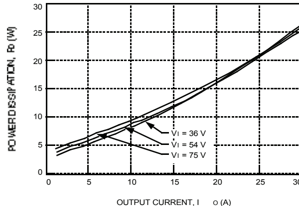
Figure 30. JW150F Power Dissipation vs. Output Current
