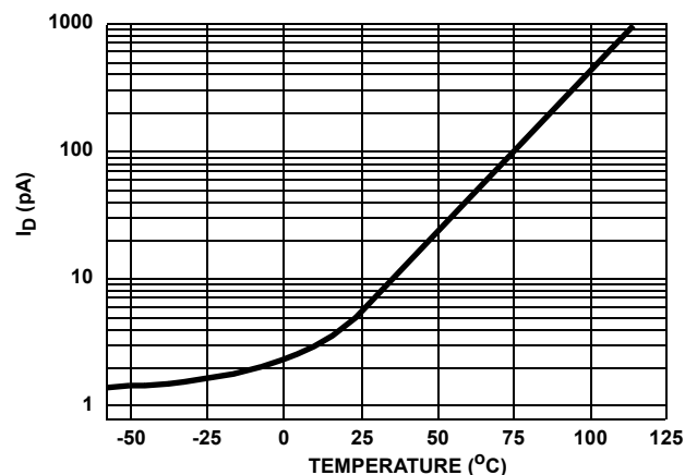
FIGURE 12. DRIFT CURRENT vs TEMPERATURE
