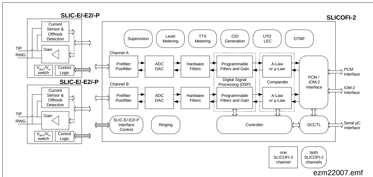
Figure 8 Line Circuit Functions included in the DuSLIC-EI-E2I-P
