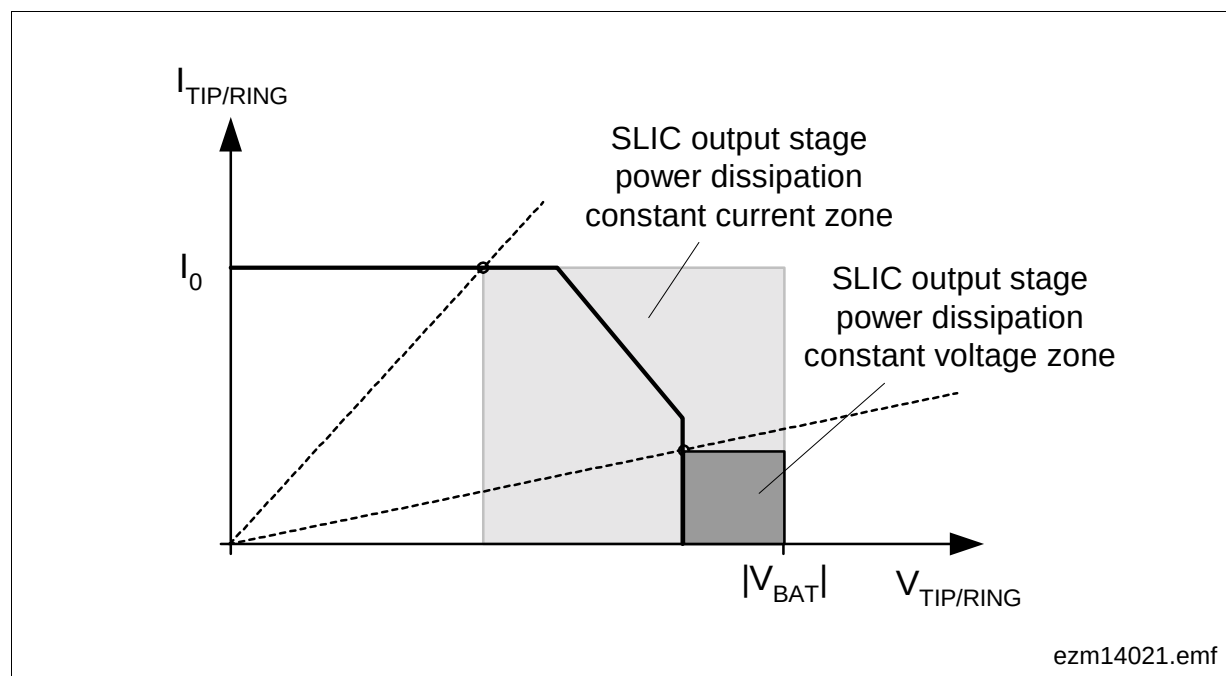
Figure 19 Power Dissipation
