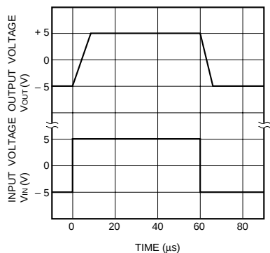
Fig.7 Output response characteristics
