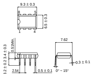
DIP8
