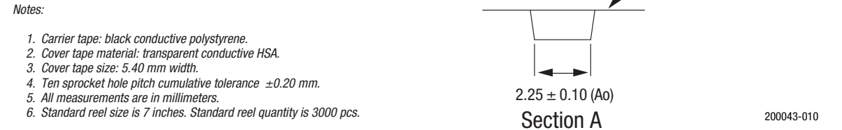
Figure 10. SC-88 Tape and Reel Dimensions
