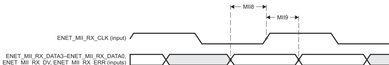
Figure 7-100. Receive Interface Timing (MII Operation)
