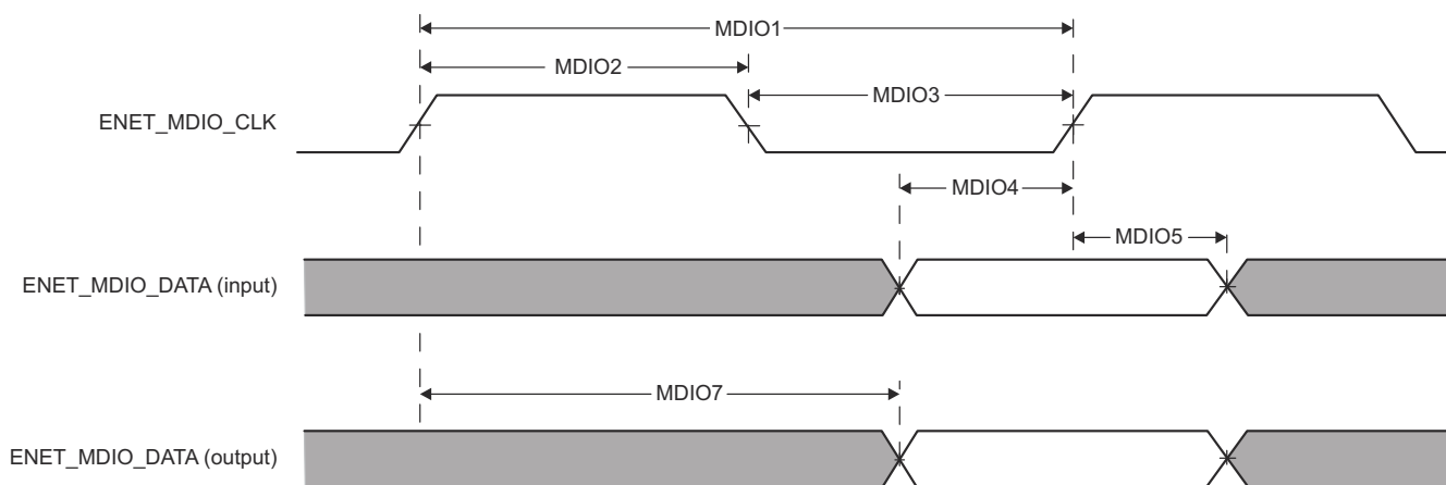
Figure 7-101. MDIO Timing Diagrams
