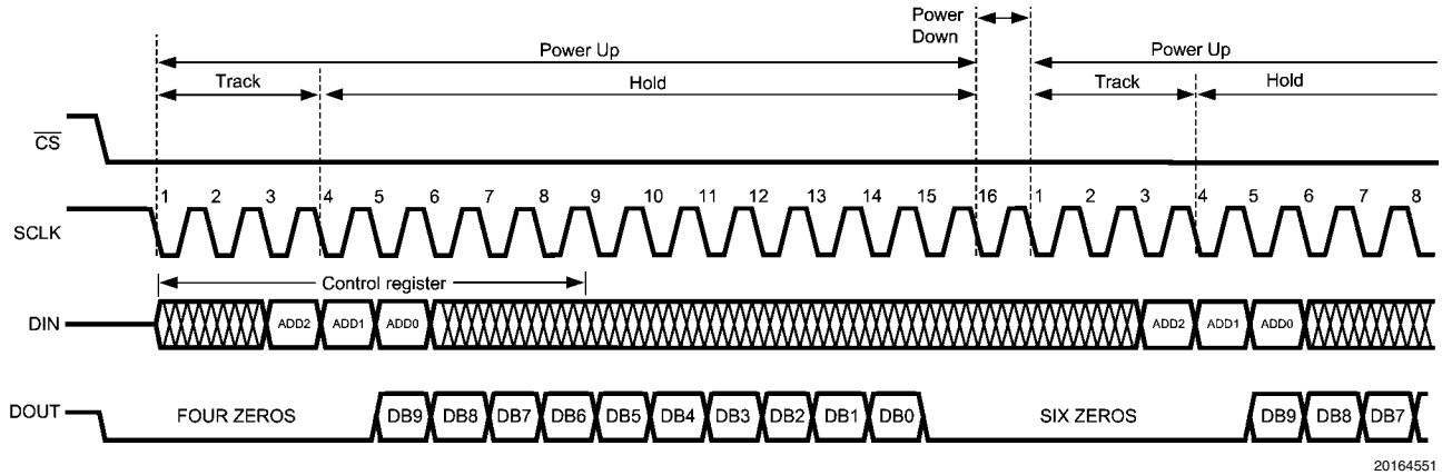
FIGURE 1. ADC108S022 Operational Timing Diagram
