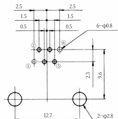
PCB mounting hole layout (Connector mounting side)
