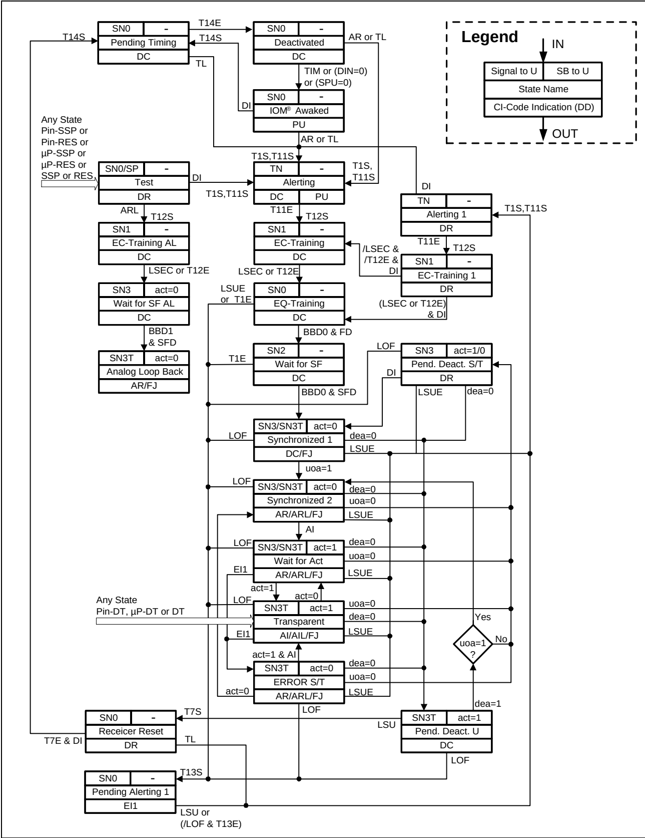
Figure 74 State Transition Diagram in NT-Auto Activation Mode
