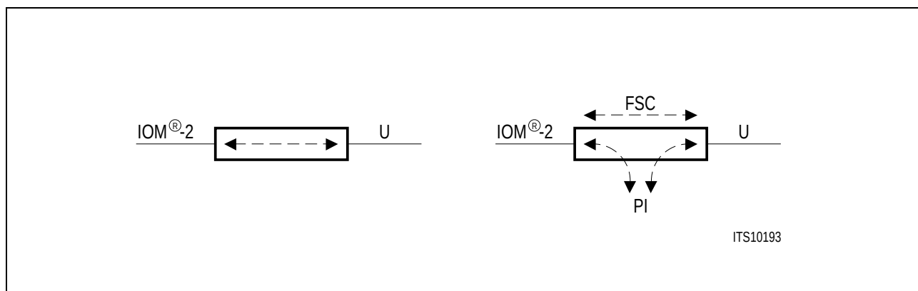
Figure 15 Stand-Alone Mode (left) and µP Mode (right)
