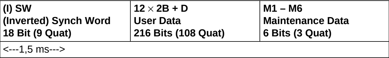
Figure 22 U-Basic Frame Structure
