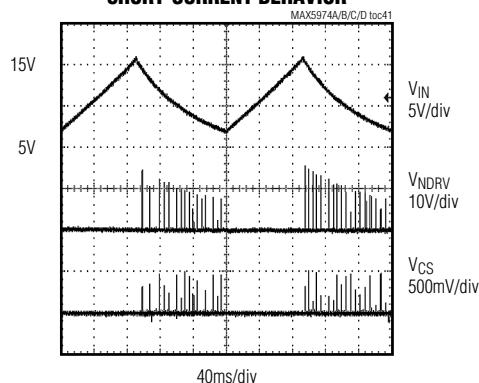
SHORT-CURRENT BEHAVIOR
