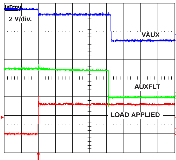
VAUX FOR VAUX OVERCURRENT
