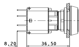
actuator with contact block
