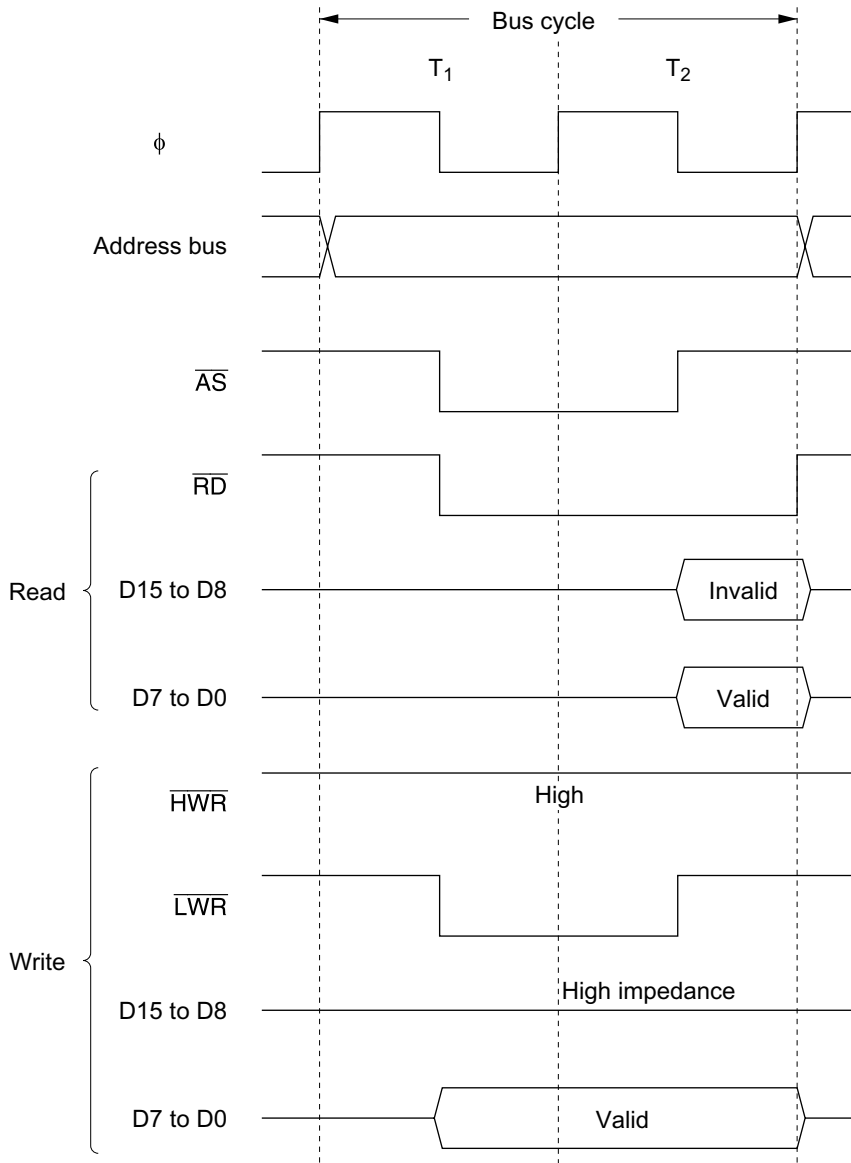
Figure 7-8 Bus Timing for 16-Bit 2-State Access Space (2) (Odd Address Byte Access)
