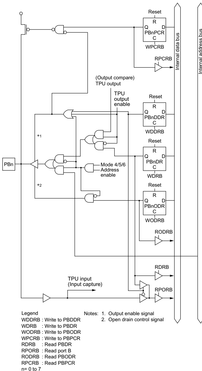
Figure C-6 Port B Block Diagram (Pins PB0 to PB7)
