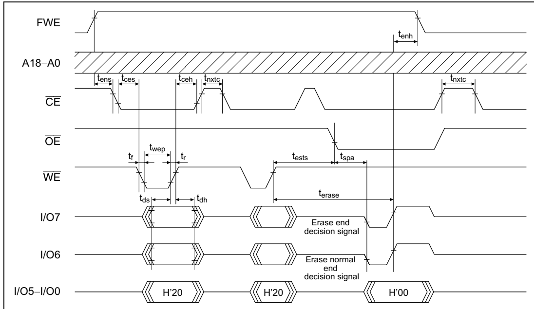
Figure 21A-23 Auto-Erase Mode Timing Waveforms
