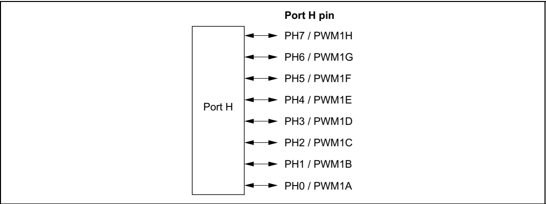
Figure 9-22 Port H Pin Functions
