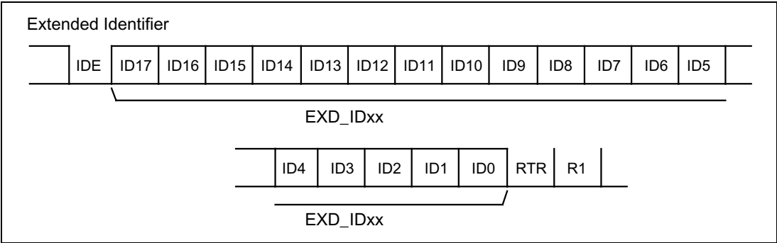
Figure 16-3 Extended identifier
