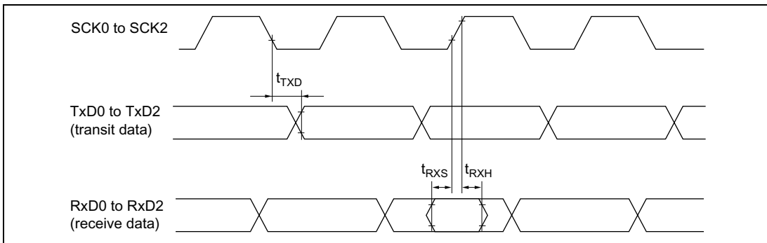
Figure 24-25 SCI Input/Output Timing (Clock Synchronous Mode)
