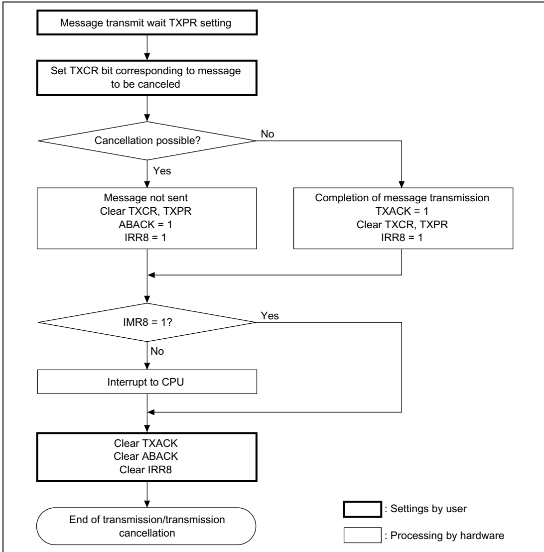
Figure 16-8 Transmit Message Cancellation Flowchart
