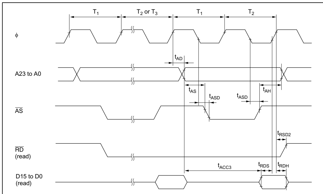
Figure 24-16 Burst ROM Access Timing (Two-State Access)
