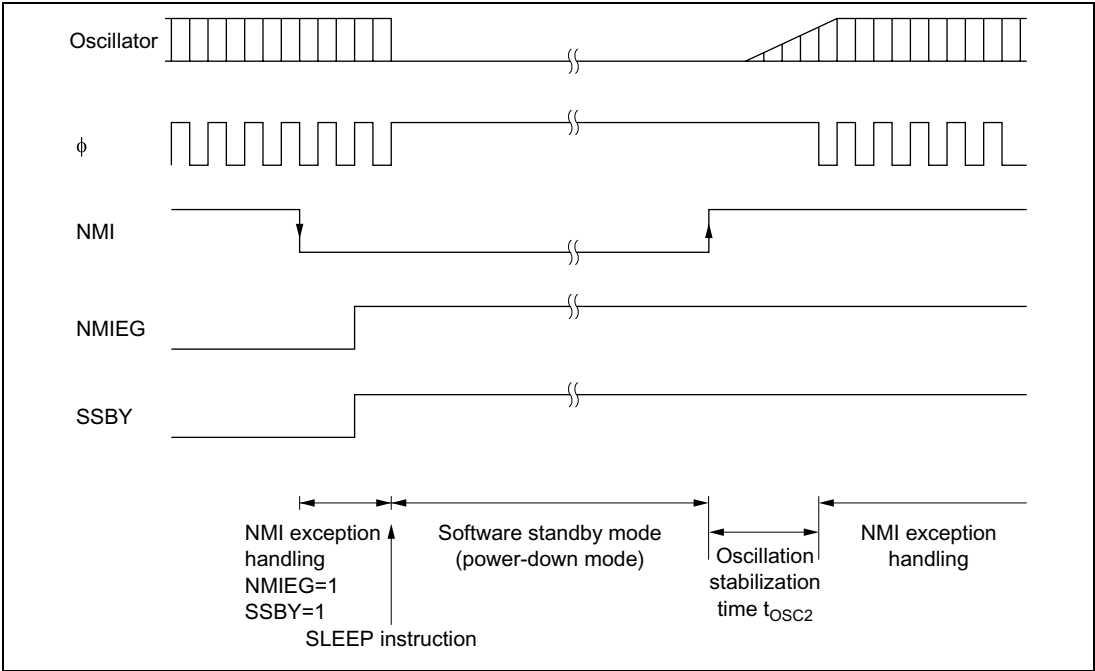
Figure 23A-3 Software Standby Mode Application Example
