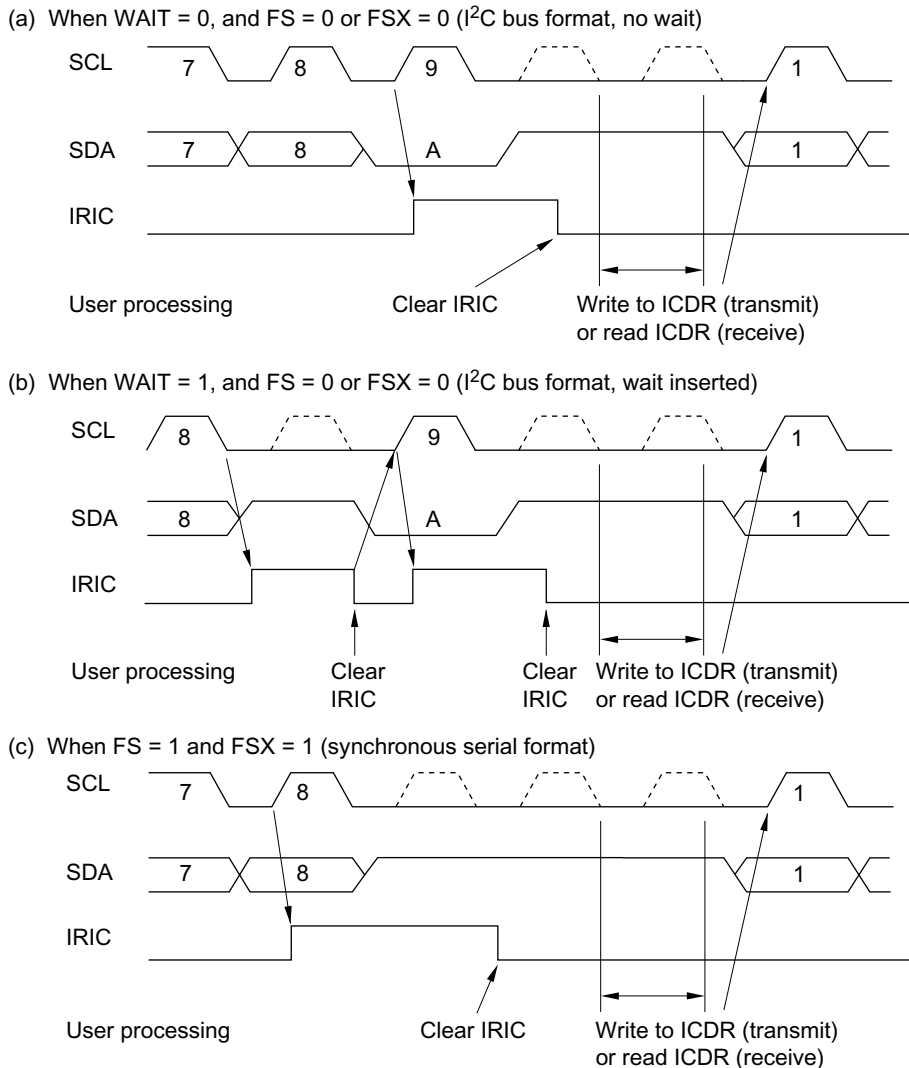
Figure 15-19 IRIC Setting Timing and SCL Control
