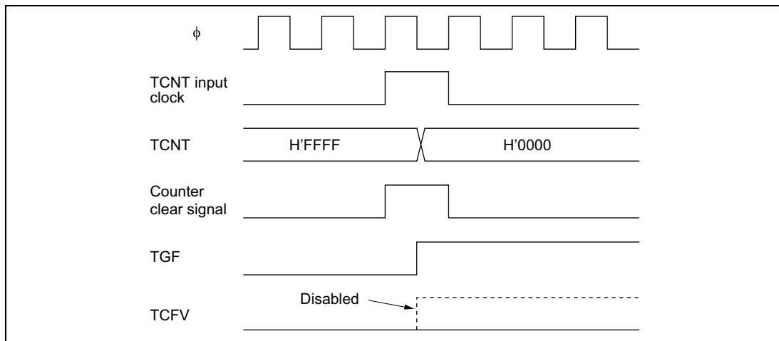
Figure 10-56 Contention between Overflow and Counter Clearing
