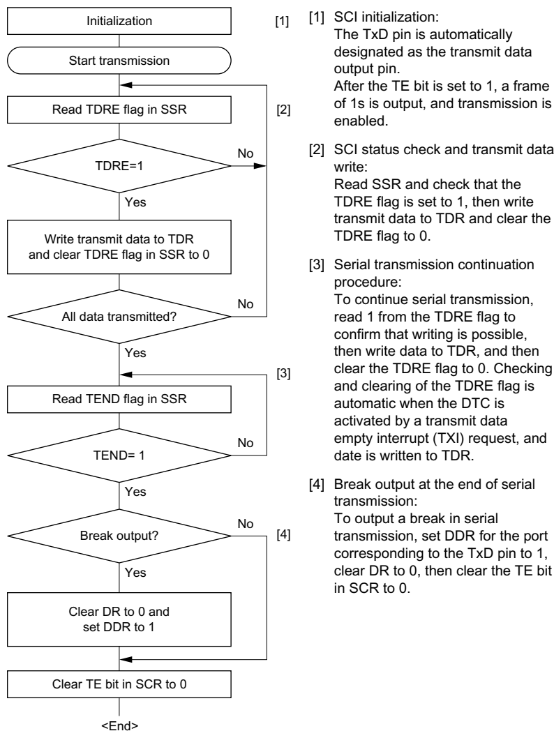
Figure 13-5 Sample Serial Transmission Flowchart
