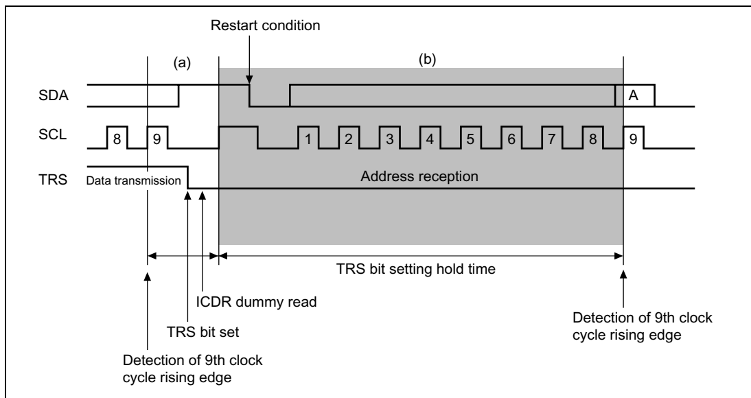
Figure 15-26 TRS Bit Setting Timing in Slave Mode
