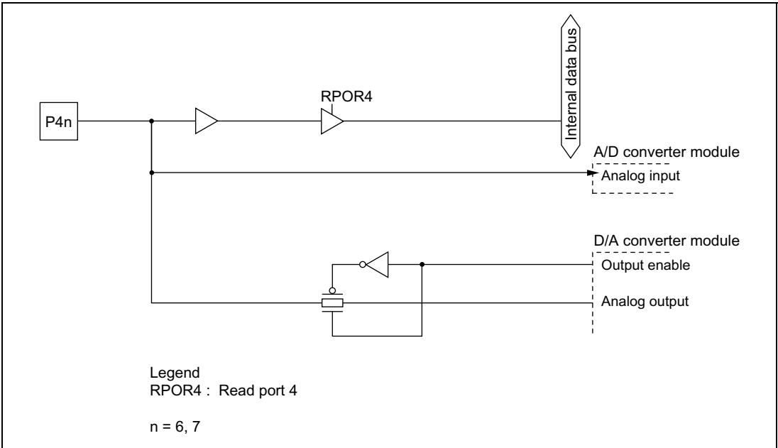
Figure C-3 (b) Port 4 Block Diagram (Pins P46, P47)
