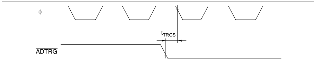
Figure 24-26 A/D Converter External Trigger Input Timing
