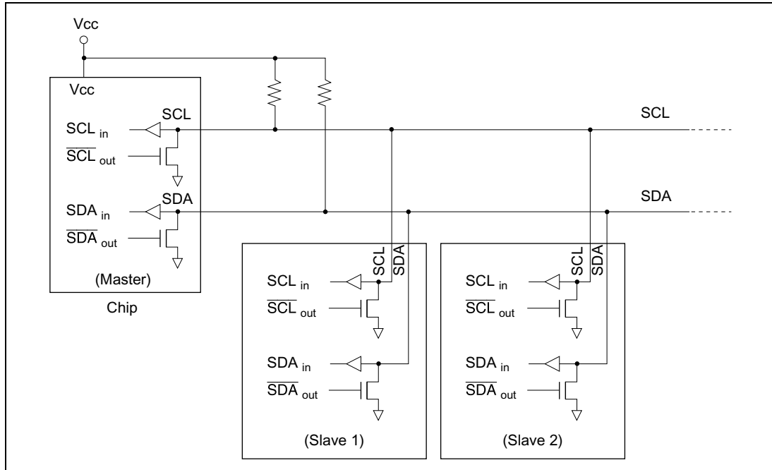
Figure 15-2 I²C Bus Interface Connections (Example: The Chip as Master)
