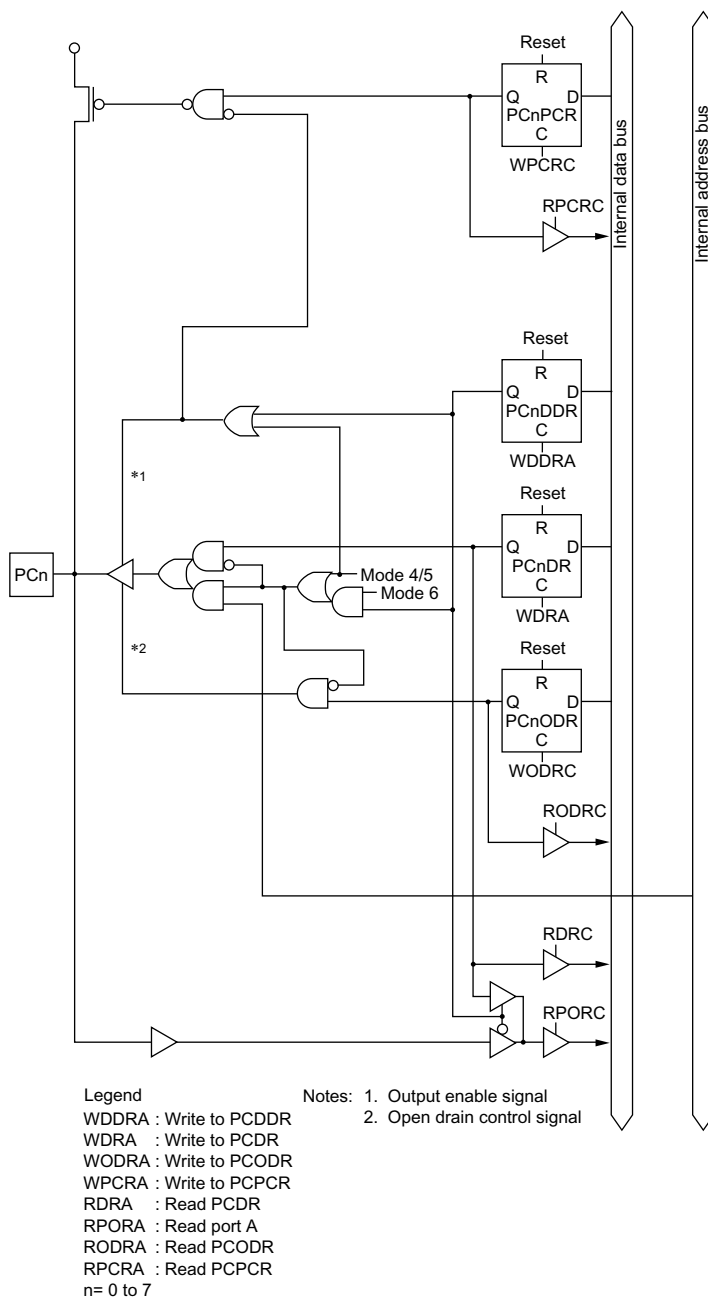
Figure C-7 Port C Block Diagram (Pins PC0 to PC7)
