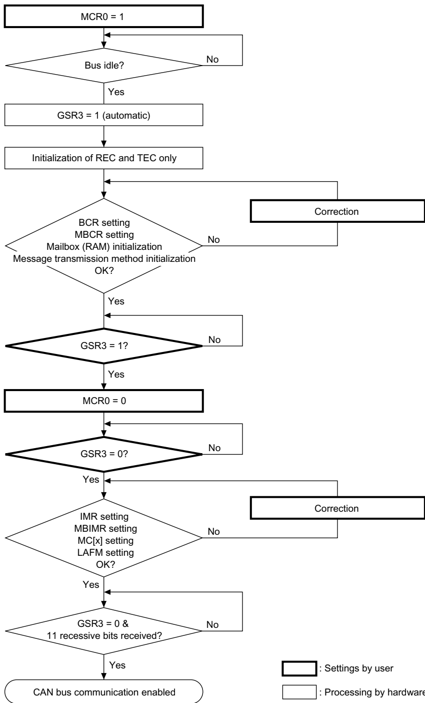
Figure 16-5 Software Reset Flowchart
