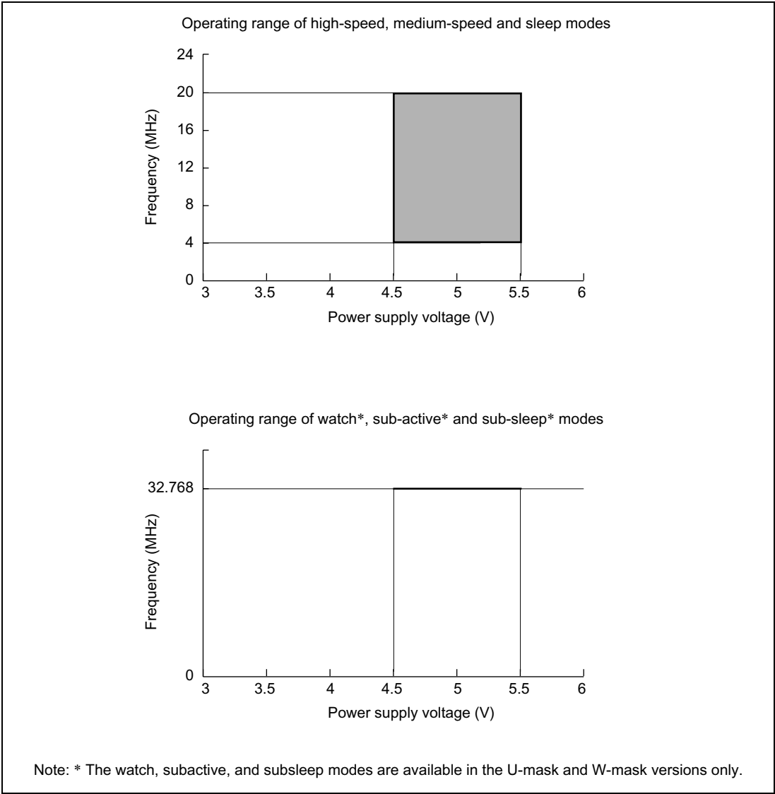
Figure 24-3 Power Supply Voltage and Operating Ranges
