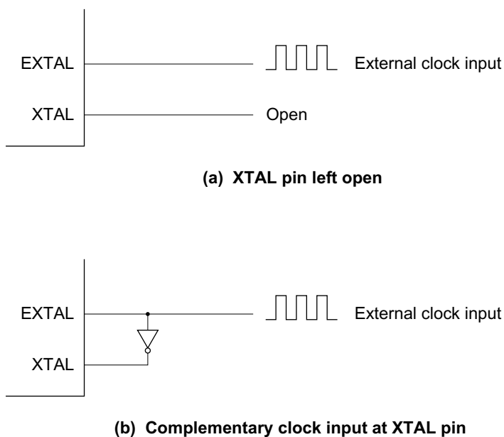
Figure 22A-6 External Clock Input (Examples)
