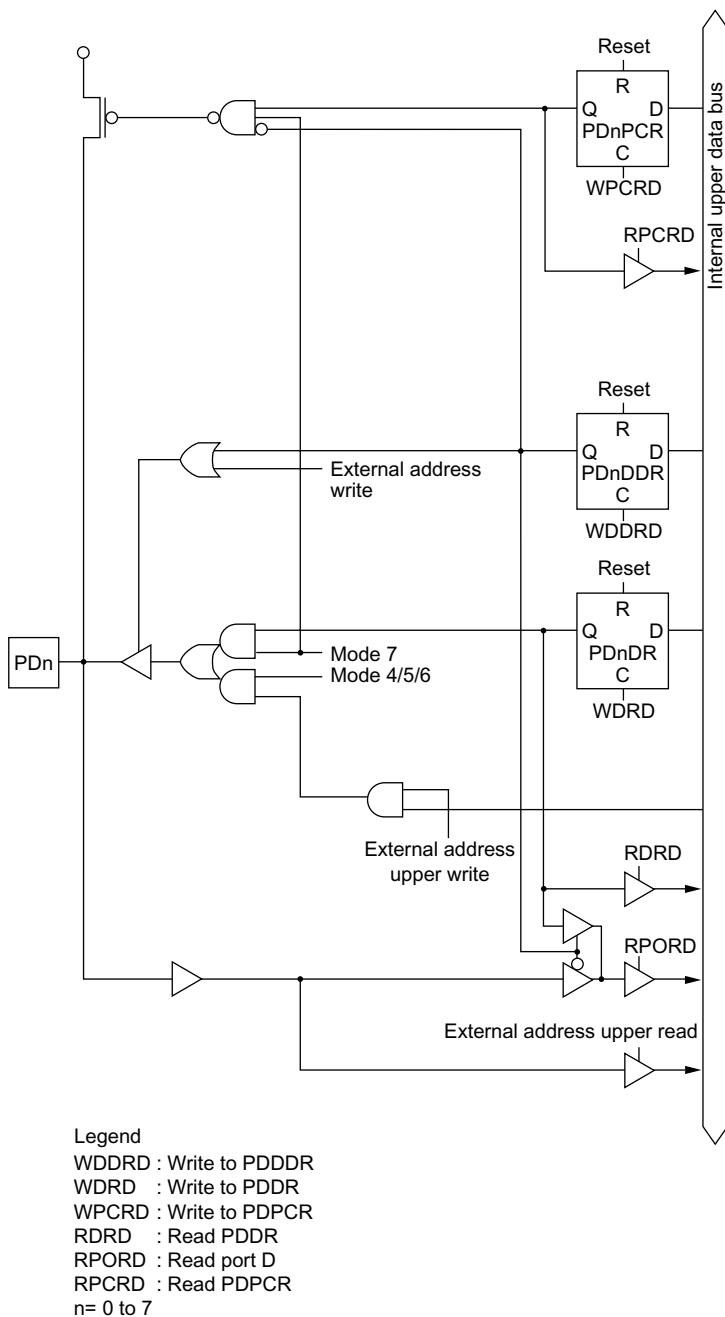
Figure C-8 Port D Block Diagram (Pins PD0 to PD7)
