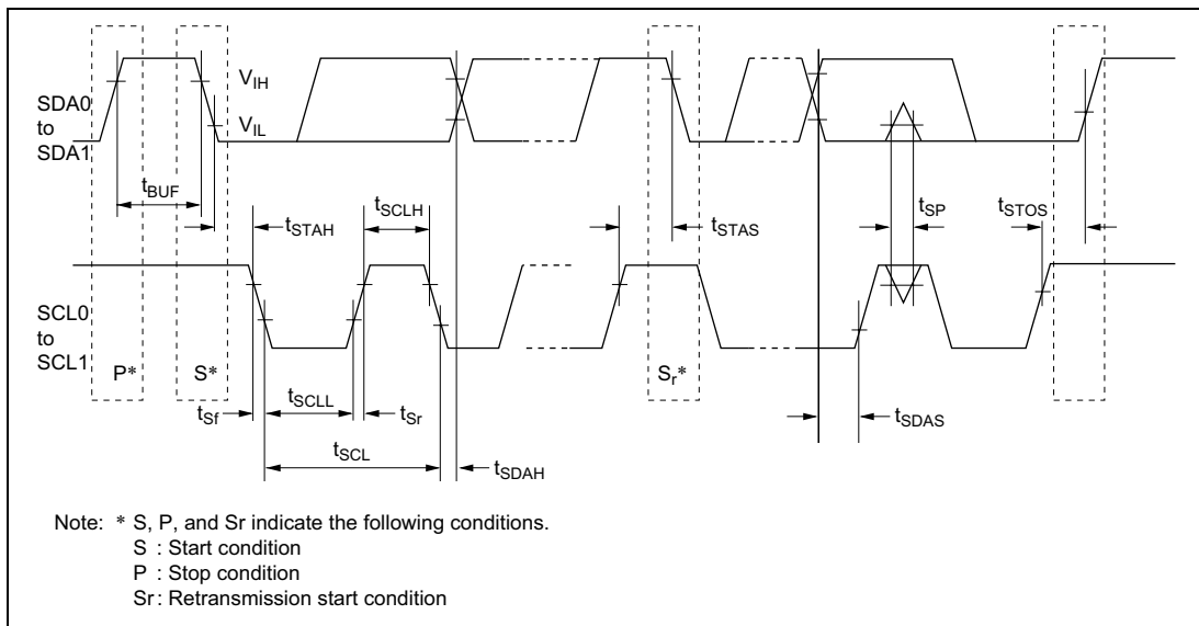
Figure 24-28 I²C Bus Interface Input/Output Timing (Option)*
