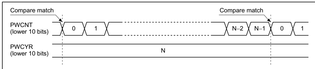
Figure 19-3 Cycle Register Compare Match
