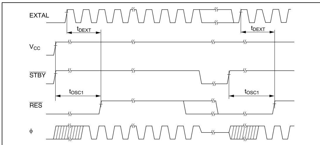
Figure 24-10 Oscillator Settling Timing
