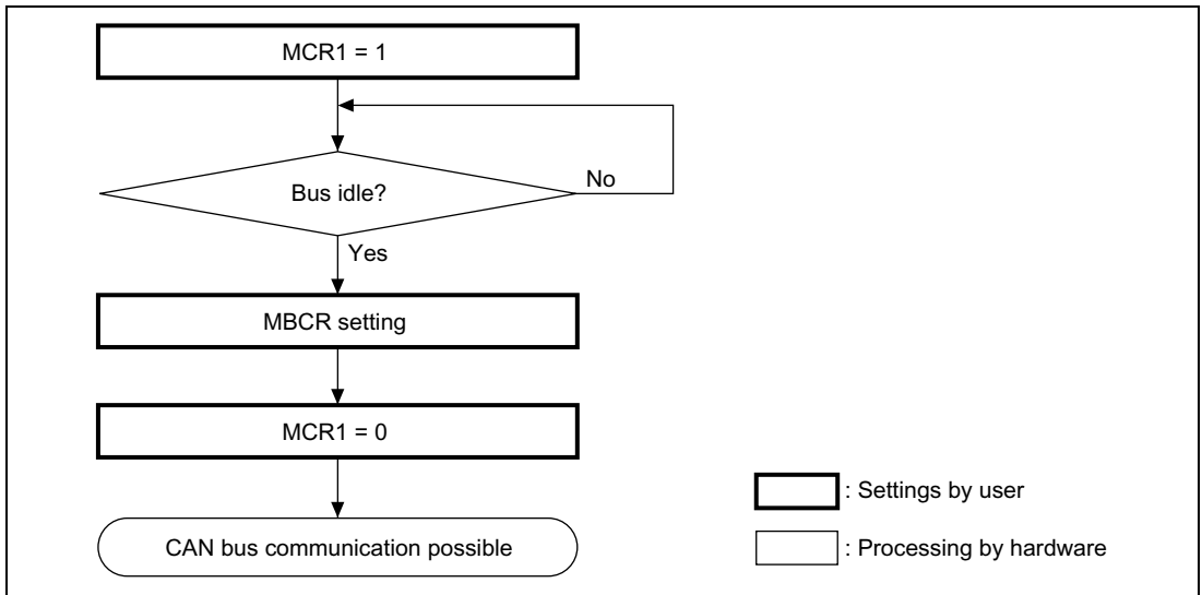
Figure 16-12 HCAN Halt Mode Flowchart
