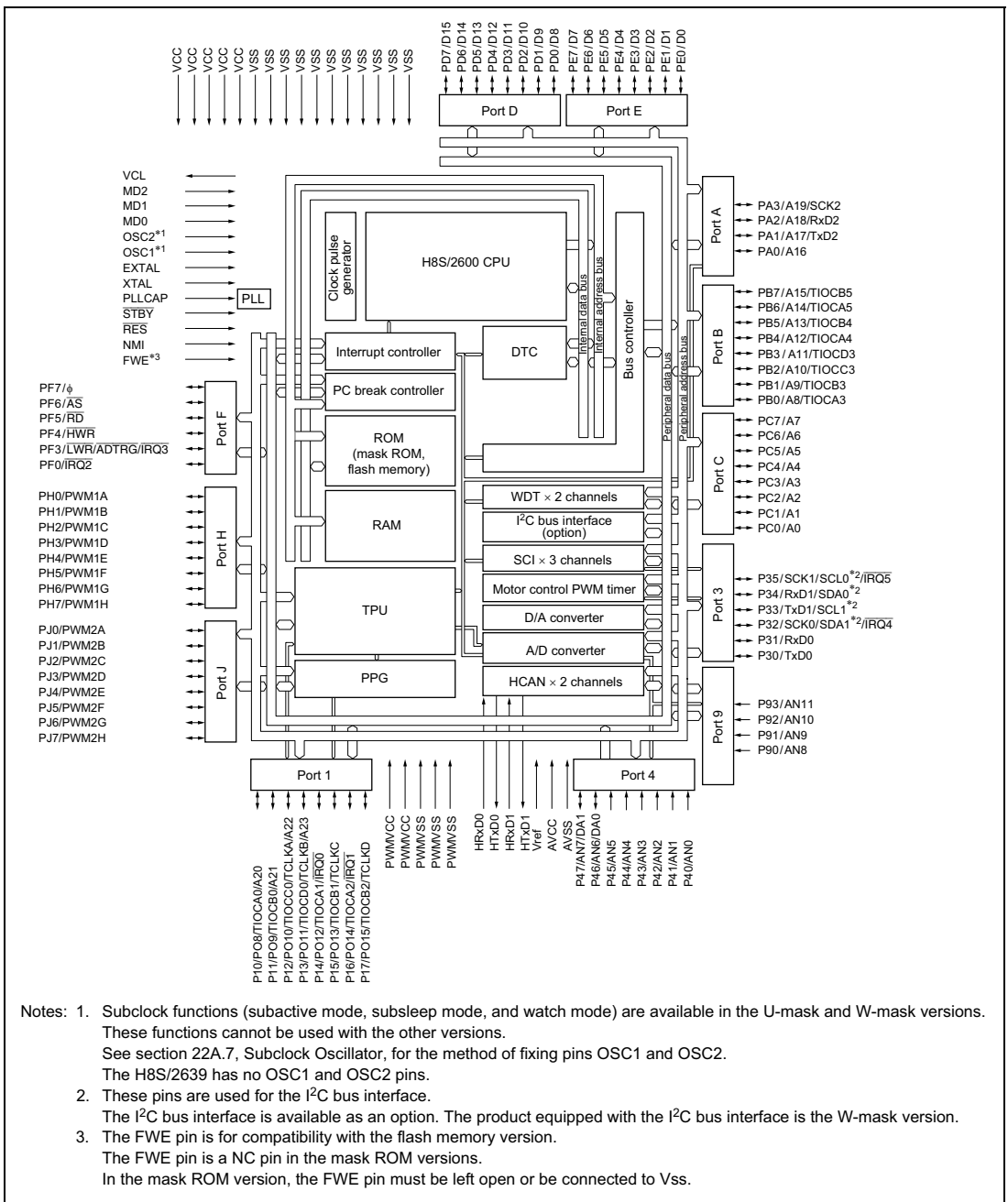
Figure 1-1 (b) Internal Block Diagram of H8S/2638, H8S/2639, and H8S/2630
