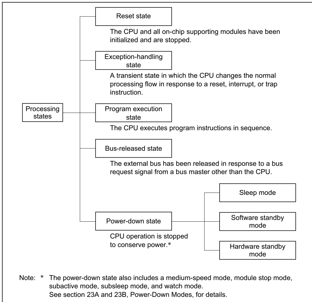
Figure 2-14 Processing States
