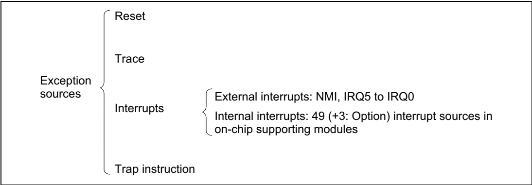
Figure 4-1 Exception Sources
