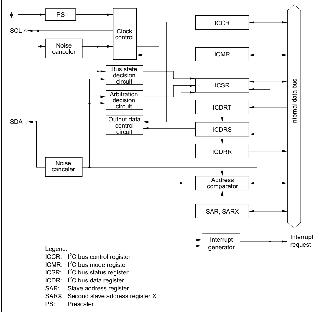
Figure 15-1 Block Diagram of I²C Bus Interface
