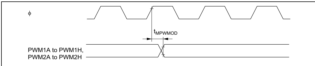
Figure 24-23 Motor Control PWM Output Timing
