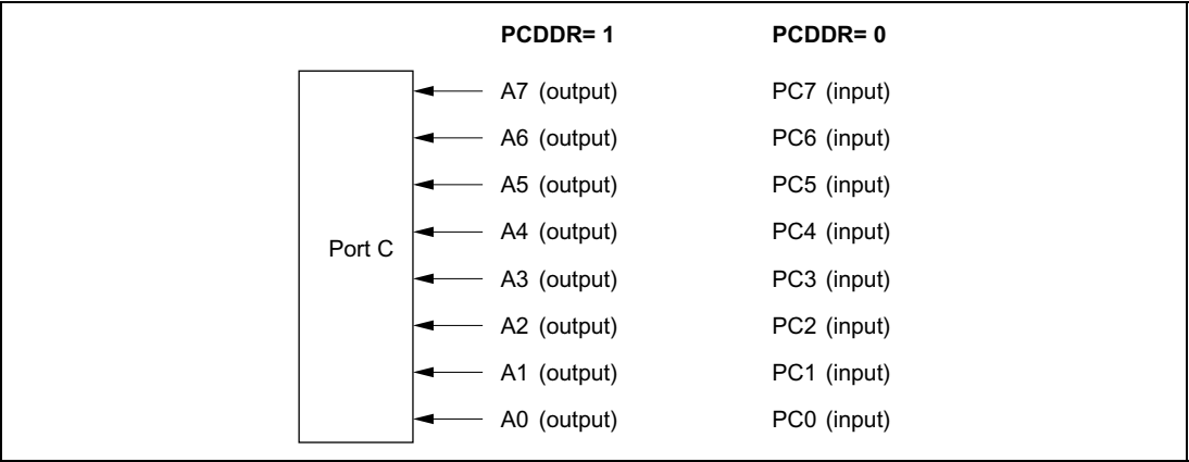
Figure 9-13 Port C Pin Functions (Mode 6)
