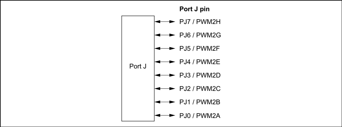
Figure 9-23 Port J Pin Functions
