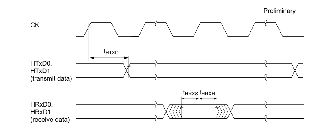
Figure 24-27 HCAN Input/Output Timing
