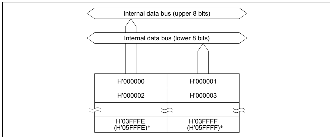
Figure 21B-1 Block Diagram of ROM 256 kbytes (384 kbytes)*
