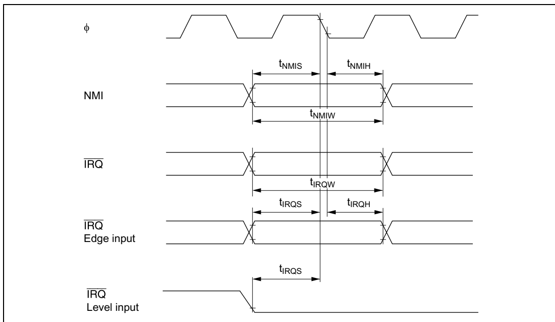
Figure 24-12 Interrupt Input Timing
