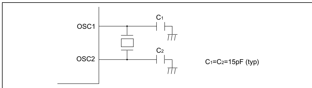
Figure 22A-8 Example Connection of 32.768kHz Quartz Oscillator
