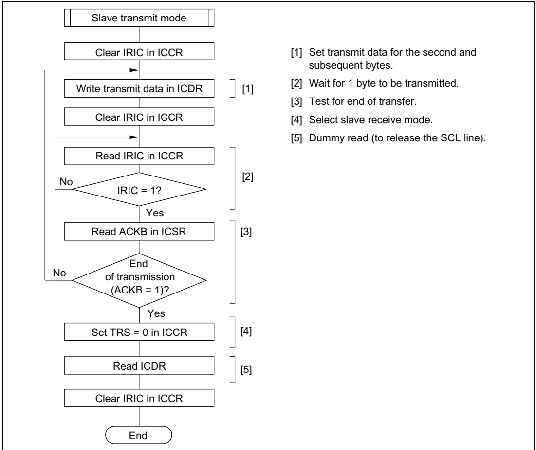
Figure 15-17 Flowchart for Slave Receive Mode (Example)
