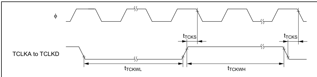
Figure 24-22 TPU Clock Input Timing
