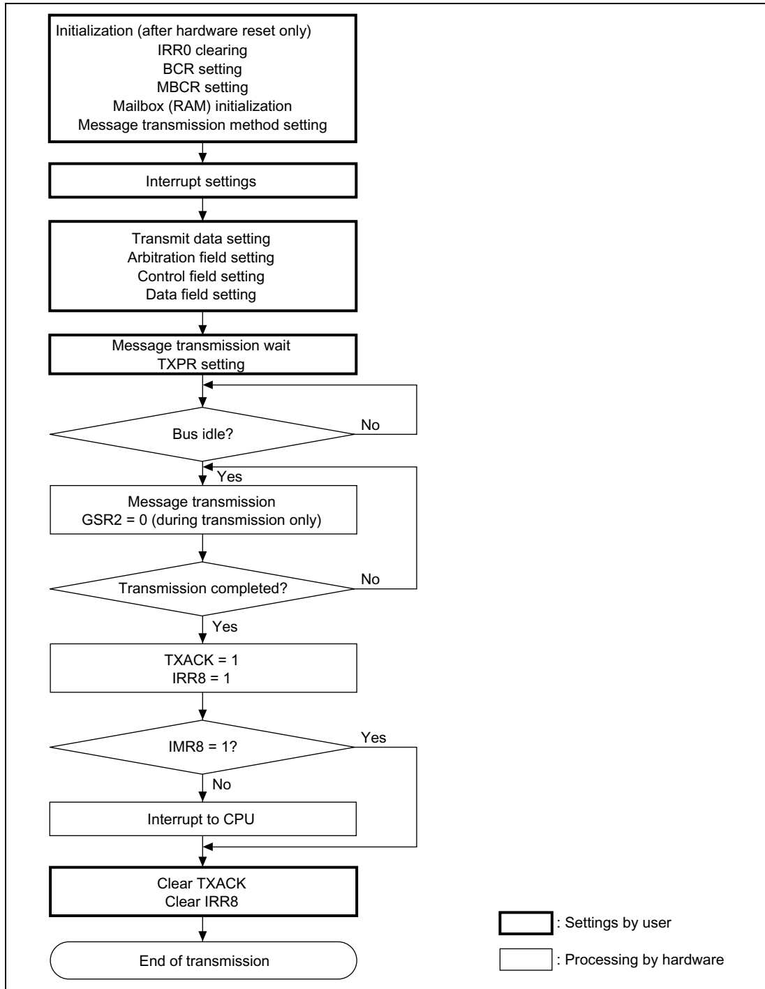
Figure 16-7 Transmission Flowchart
