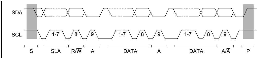
Figure 15-5 I 2 C Bus Timing
