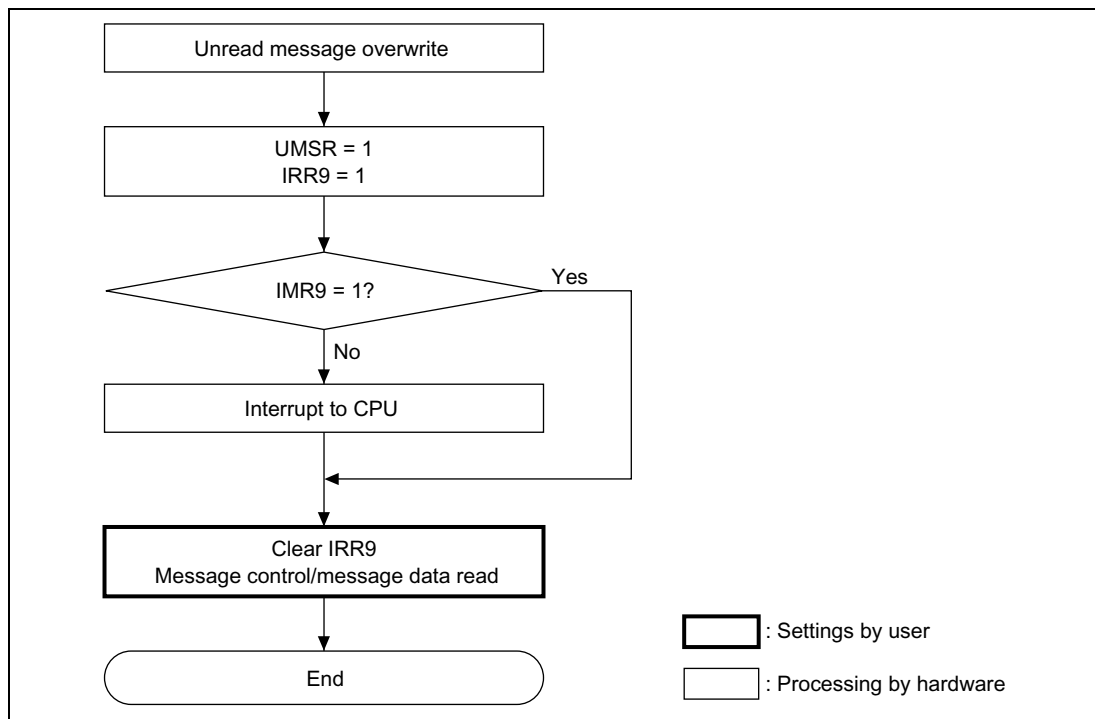
Figure 16-10 Unread Message Overwrite Flowchart
