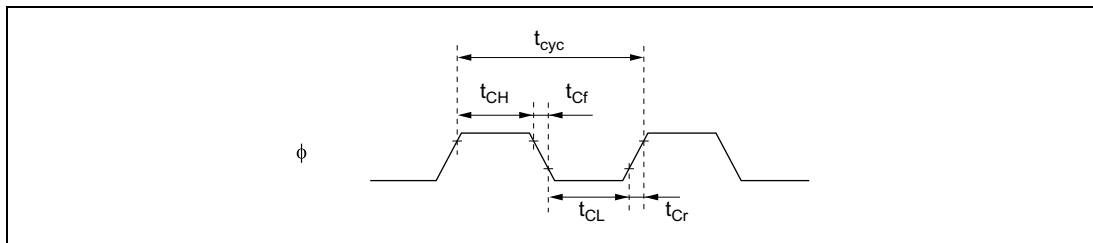
Figure 24-9 System Clock Timing
