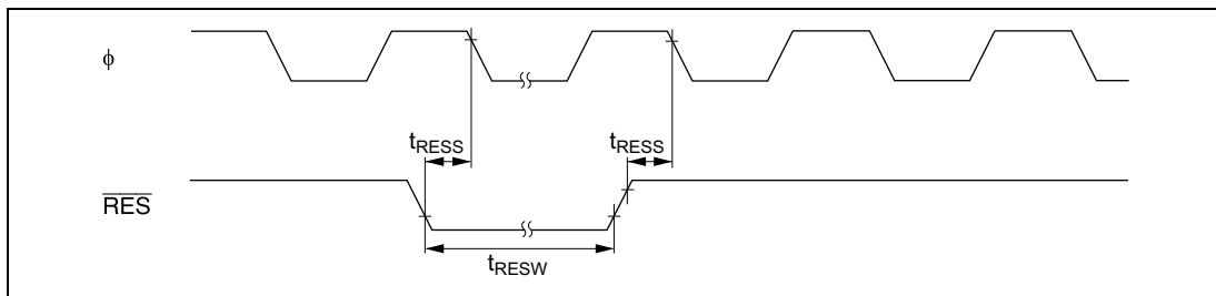
Figure 24-11 Reset Input Timing
