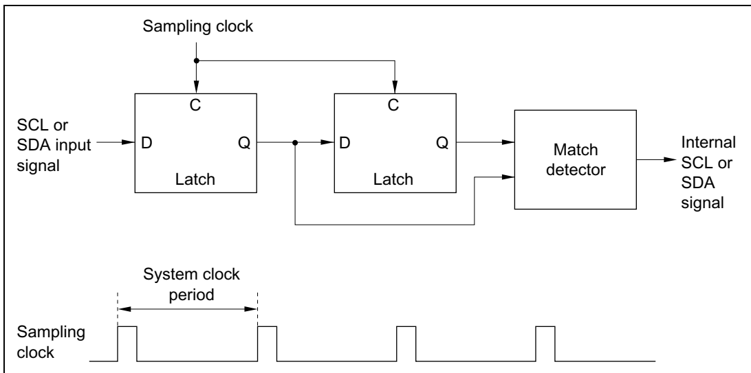
Figure 15-20 Block Diagram of Noise Canceler
