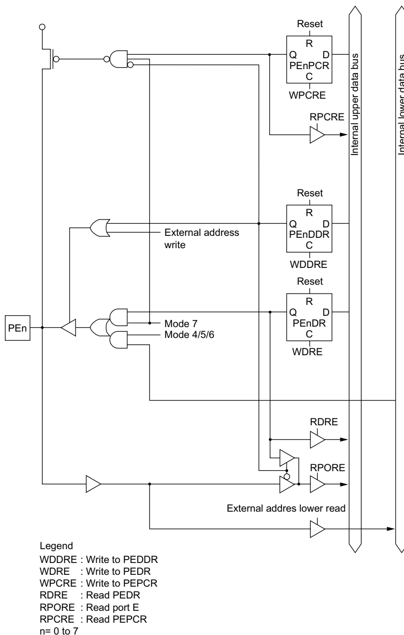
Figure C-9 Port E Block Diagram (Pins PE0 to PE7)
