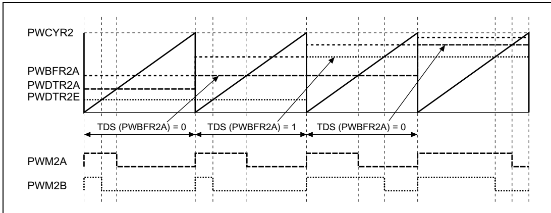
Figure 19-11 PWM Channel 2 Operation
