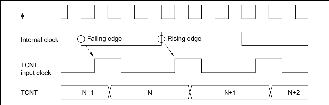
Figure 10-34 Count Timing in Internal Clock Operation
