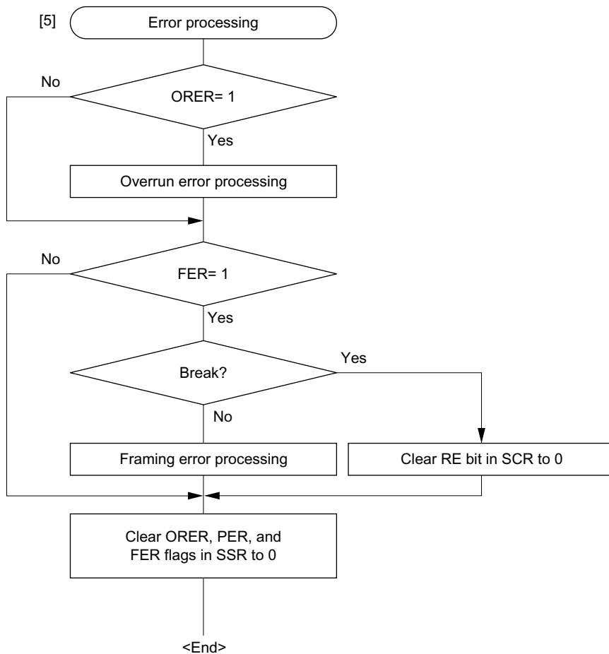
Figure 13-12 Sample Multiprocessor Serial Reception Flowchart (cont)
