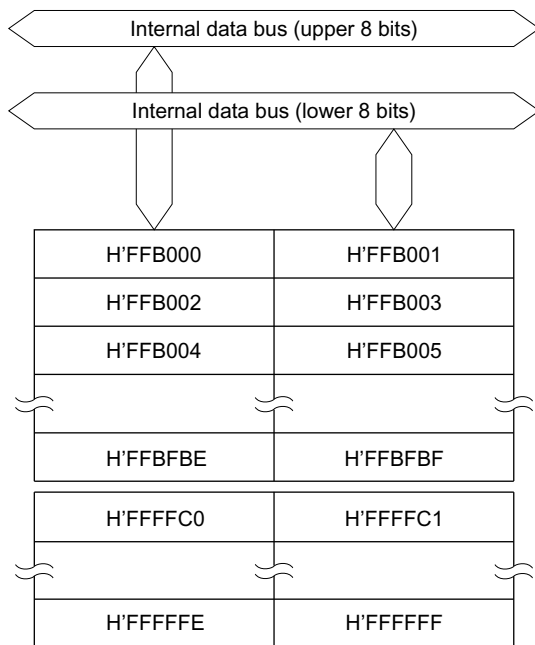
Figure 20-1 (b) Block Diagram of RAM (H8S/2638, H8S/2639, and H8S/2630)
