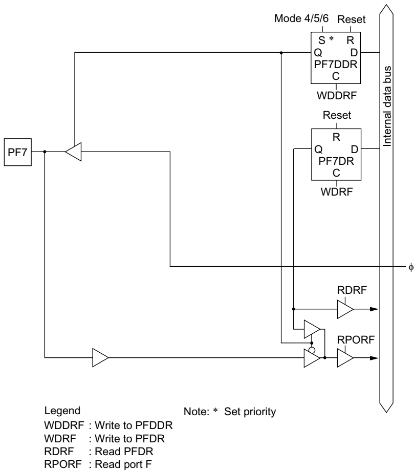
Figure C-10 (f) Port F Block Diagram (Pin PF7)
