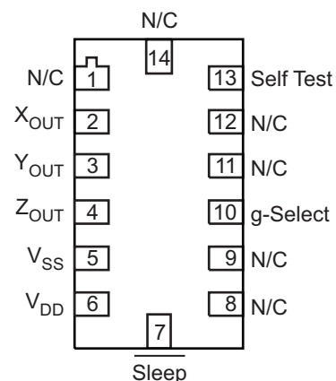
Figure 1. Pin Connections
