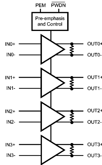
20188903 DS15BR401 Block Diagram
