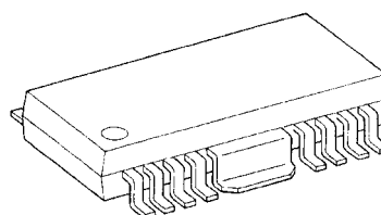
HSOP16-P-300-1.00
