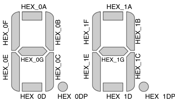
Figure 2–4. Pin-Out Diagram for the Dual 7-Segment Display
