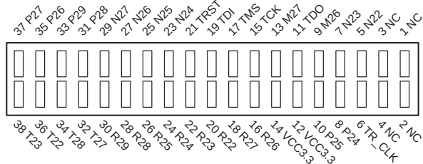
Figure 2–8. Debug Mictor Connector - J20
